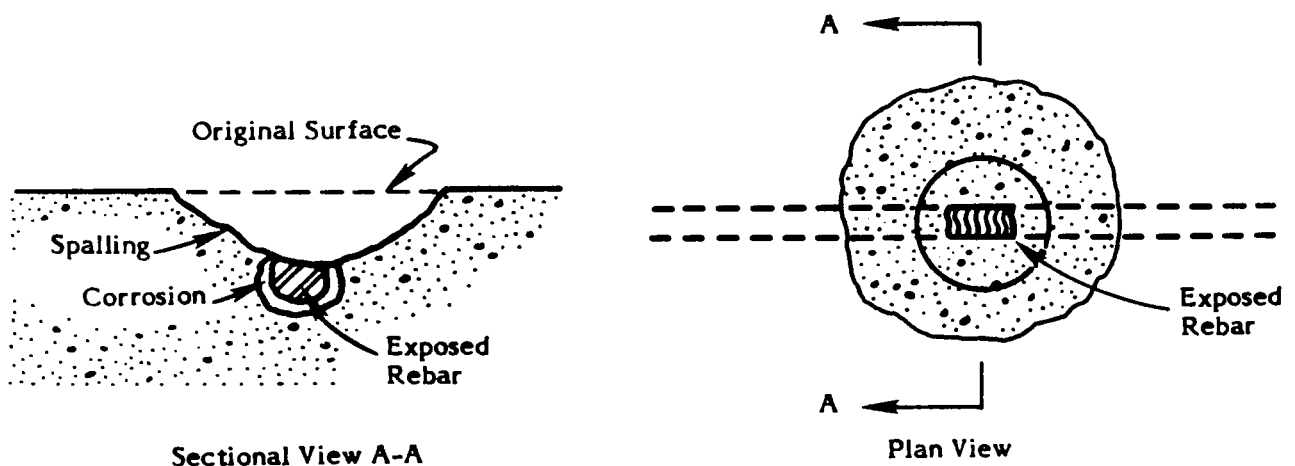
FIGURE II-10. CONCRETE DETERIORATION DUE TO METAL CORROSION
