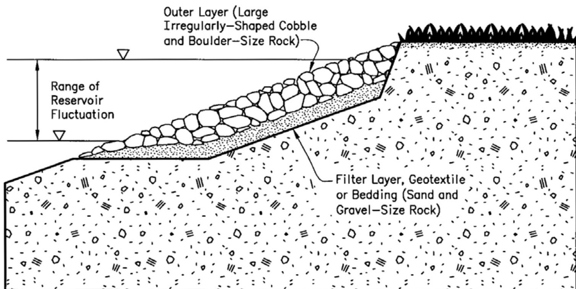
FIGURE II-14. RIPRAP
